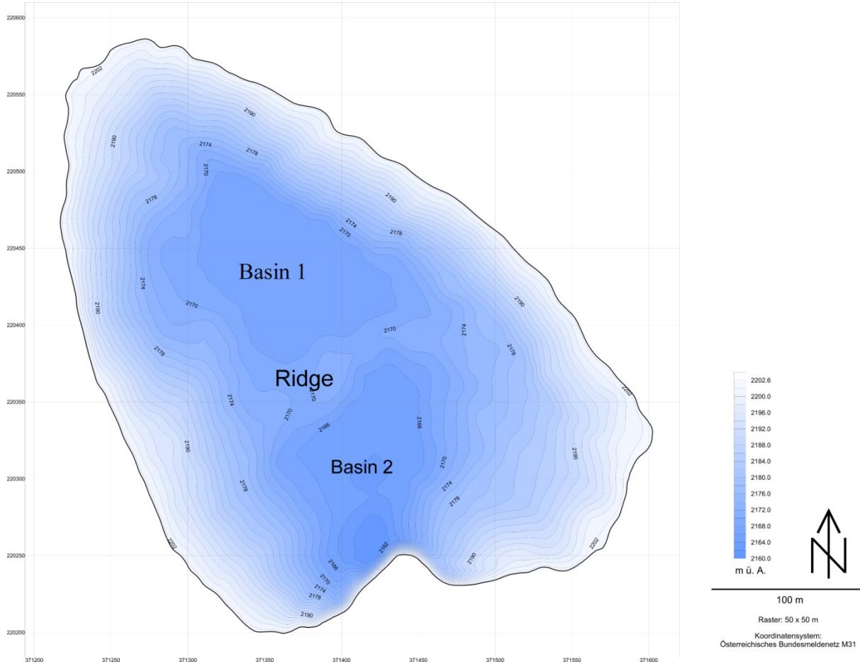
Figure 4: Bathymetry map of Obersulzbach See
