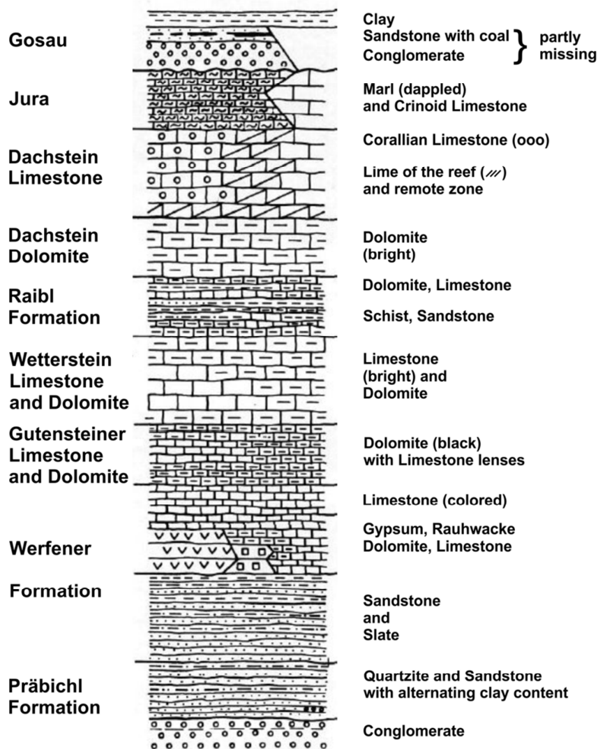
Figure 3.4: Stratigraphic scheme of the Gesäuse Mountains (after Büchner, 1970, p. 9).
