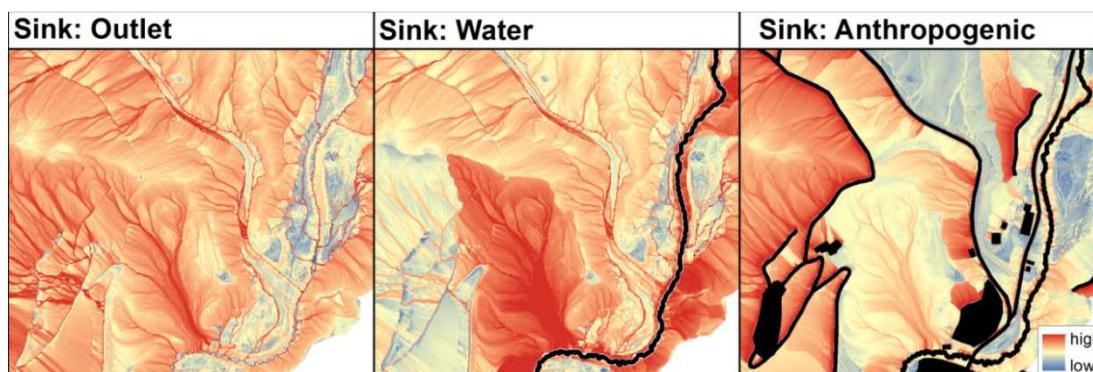
Figure 4.4: Clip (0.4 x 0.4 km) of the Oberwölz catchment showing the connectivity routing (from low (blue) to high (red)) for different sinks (in black) on the base of the original Airborne Laserscan (ALS) DEM. The outlet-sink itself is not shown in the picture.
