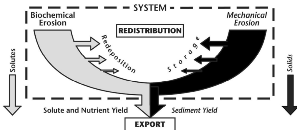
Figure 2.13: Weathering, erosion and denudation as a mass balance problem (after Slaymaker, 2003).
