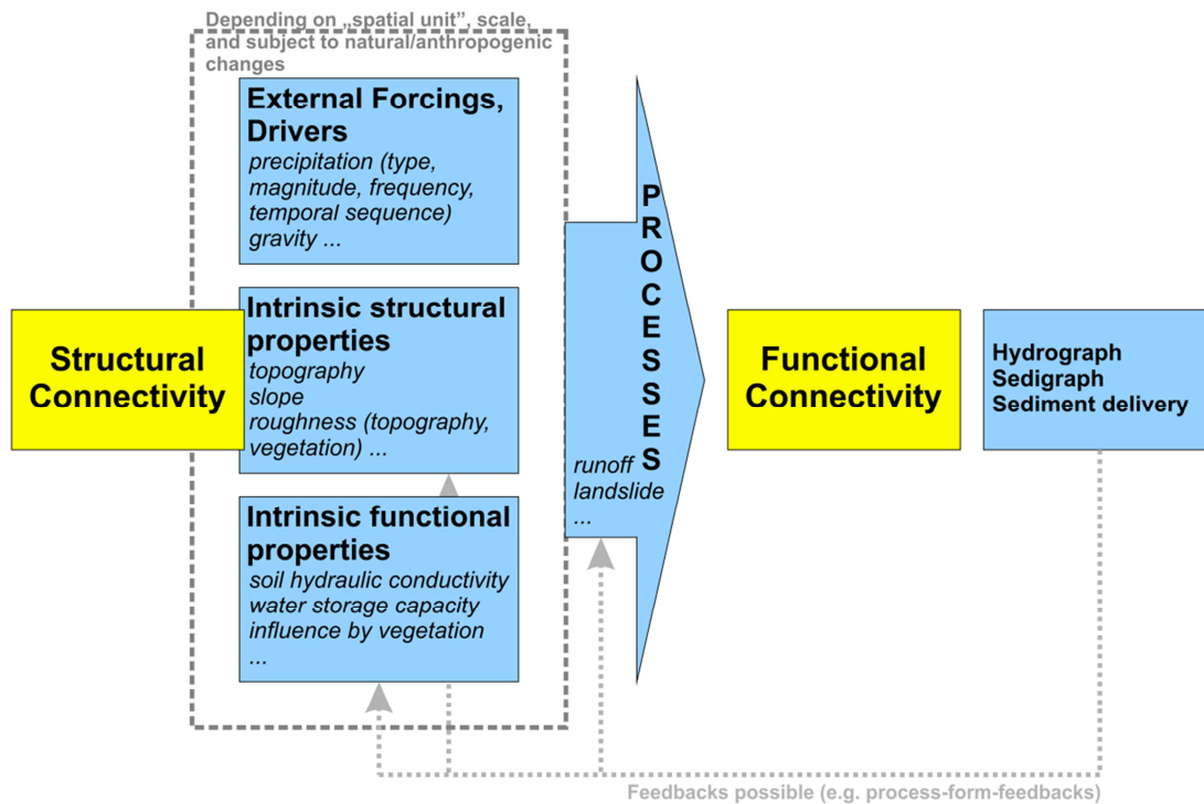
Figure 2.14: Conceptual model of water or sediment connectivity, influencing factors and drivers (after Heckmann et al., 2018).
