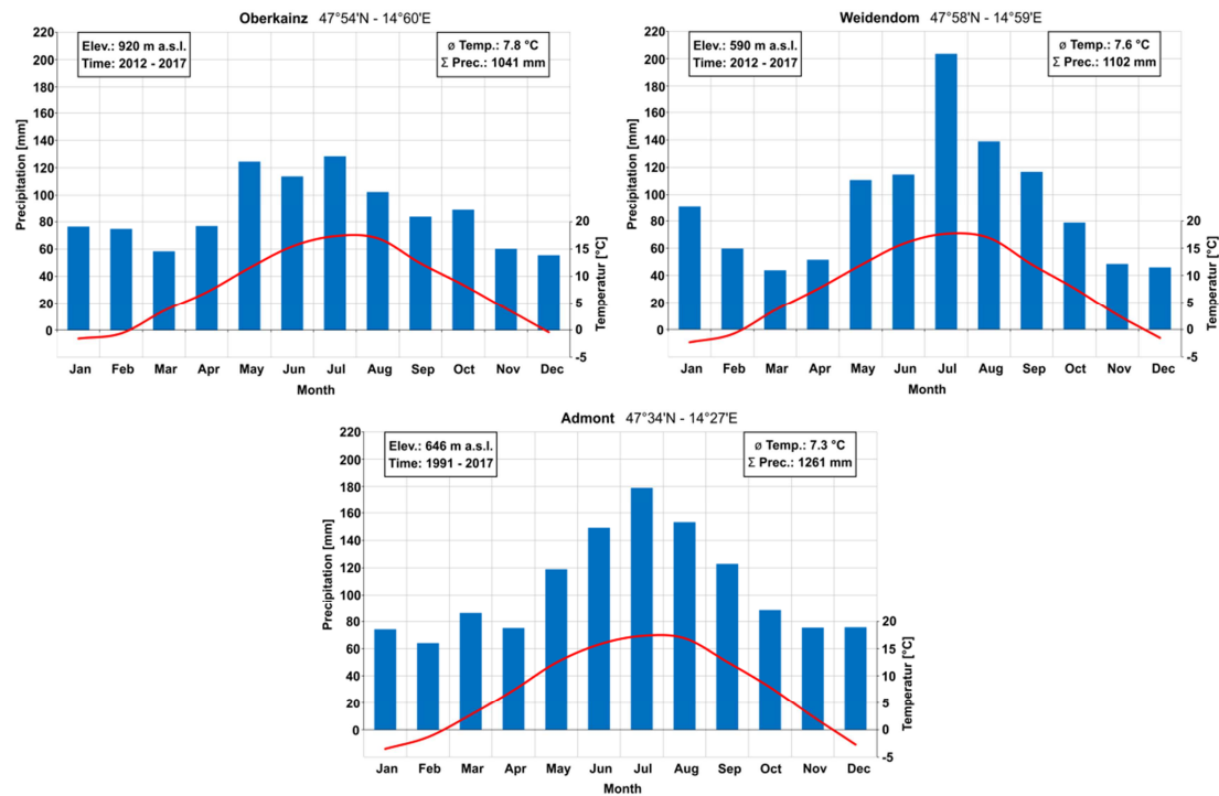
Figure 3.7: Climate diagrams of the Gesause region: (top left) Oberkainz, (top right) Weidendom and (bottom) Admont (for location see Figure 3.1). The red curve represents the annual course of the temperature and the blue columns represent the monthly precipitation. Note: for Oberkainz and Weidendom snow is not considered in the precipitation amounts. Elev. = elevation, Time = observation period, \bar{\theta} Temp. = mean annual temperature, \Sigma Prec. = mean annual amount of precipitation.
