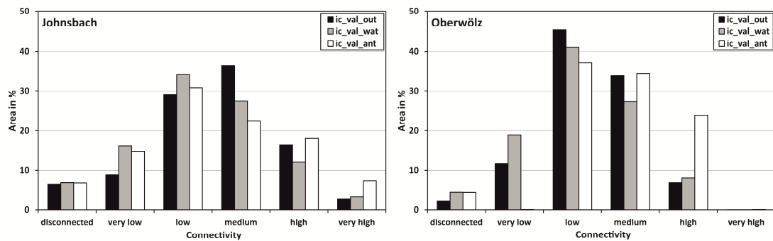
Figure 4.8: Catchment areas of Johnsbach and Oberwölz divided into connectivity classes for three scenarios using the Valley DEM and the targets: outlet (black), water (grey), and anthropogenic (white).
