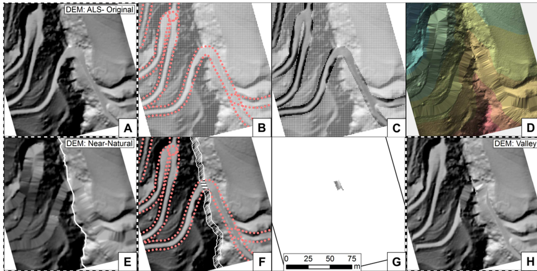
Figure 4.5: Exemplary flowchart of the generation of the different DEMs. Hillshades are in the background for better understanding, (A) the original LIDAR-based DEM, (B) conversion of the raster-data to a point cloud and buffering (5 m) of the digitized road dataset (red outlined polygon), (C) cutting out the points intersecting with the road-buffer file, (D) generating a TIN out of the remaining point cloud, (E) converting the TIN to a raster-dataset, the new Near-Natural DEM and calculating the new flow-accumulation on that base, respectively the new channel network (white line), (F) buffering (3 m) the channel network and intersecting it with the buffered road dataset, (G) using the intersection-file as clip-mask to extract these areas from the Near-Natural DEM and (H) imprint it onto the ALS DEM and creating the Valley DEM.
