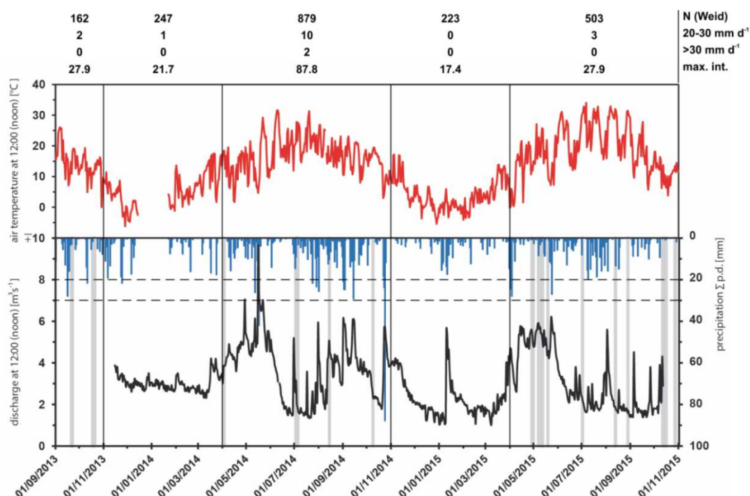
Figure 5.3: Precipitation and temperature (recorded at Weidendom) as well as river discharge (recorded at Gseng Bridge) during the observation period; gray stripes indicate the time of the scan campaigns; black vertical solid lines indicate summer/winter seasons; black horizontal dashed lines mark the threshold interval for precipitation. Parameters on top are given for the indicated season in the order from top to bottom: total precipitation in mm; number of days with 20-30 mm d -1 ; number of days with >30 mm d -1 ; maximal daily intensity.
