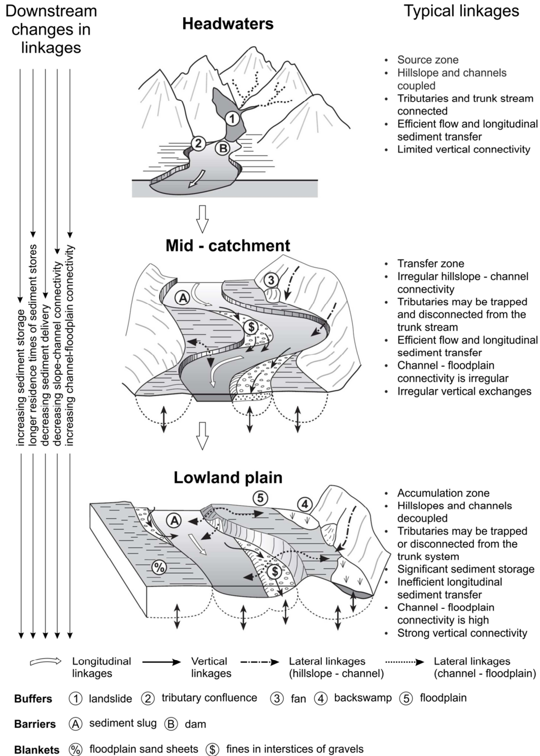
Figure 2.16: Spatial dimensions of landscape connectivity in an idealized catchment. Patterns of longitudinal, lateral and vertical linkages have different strength in headwater, mid-catchment and lowland plain settings. This is largely dependent on the configuration of each process zone and the location of blockages in the system (modified from Brierley and Fryirs, 2005).
