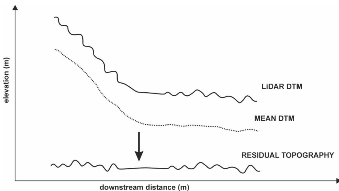
Figure 4.3: One-dimensional example of the residual topography calculation. The dotted line is the profile of the mean DEM calculated over the LiDAR DEM (continuous line) with a neighborhood analysis approach. Residual topography is calculated as the difference between LiDAR DEM and mean DEM (Cavalli et al., 2008).
