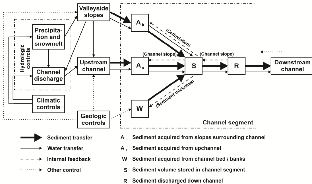
Figure 2.5: The stream channel sediment budget (after Caine, 1974).
